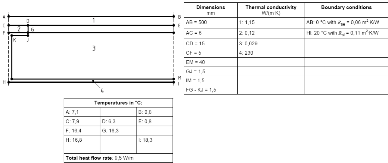
Figure 3. Test reference case 2 as listed in EN ISO 10211:2017
