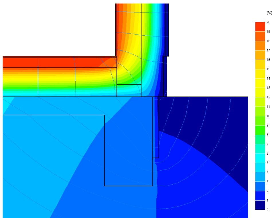
Figure 8: Isotherms (increment 1 °C) and heat flow lines (increment 0.5 W/m) (zoomed view).
