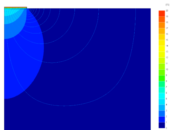
Figure 7: Isotherms (increment 1 °C) and heat flow lines (increment 0.5 W/m)
