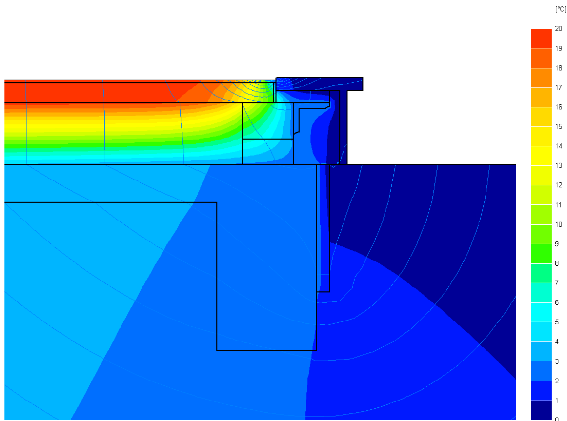
Figure 9: Isotherms (increment 1 °C) and heat flow lines (increment 0.5 W/m) (zoomed view).
