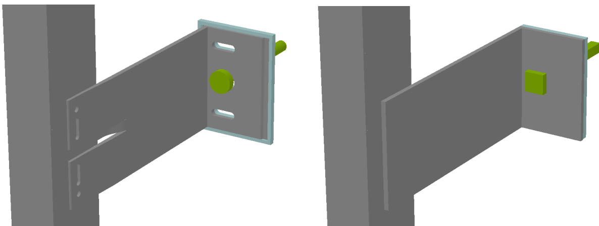
Figure 5 Full detail (left) and Simplified (right)
