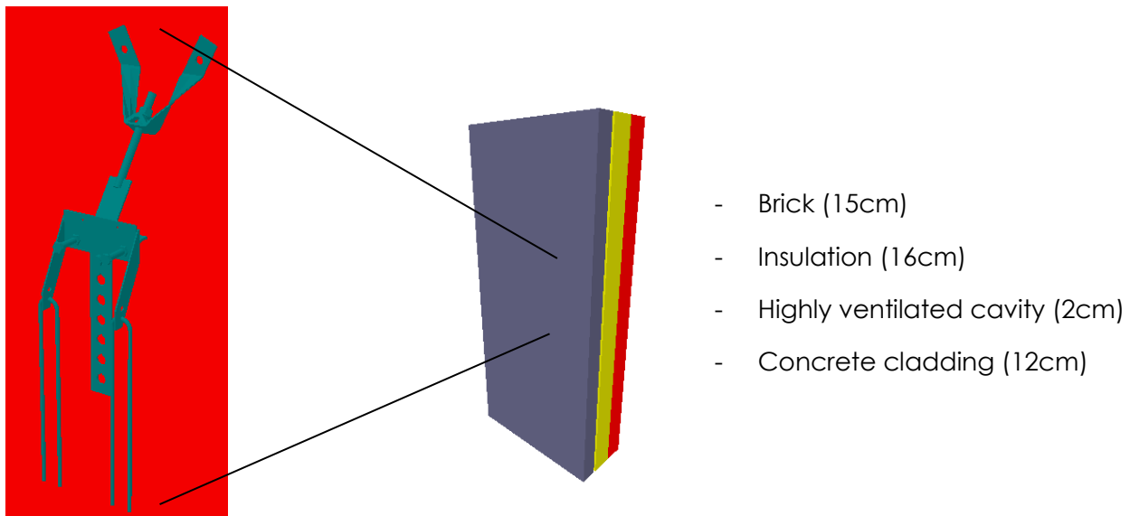
Figure 1 Model of the ventilated façade
