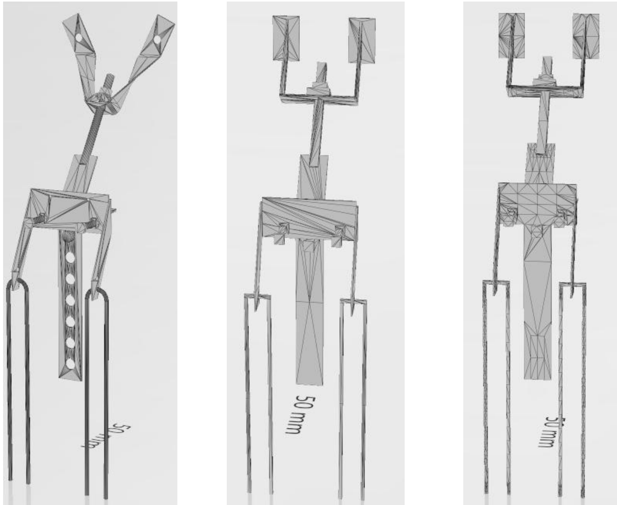
Figure 2 Anchor variations: Full detail (left), Simplified 1 (middle), Simplified 2 (right)
