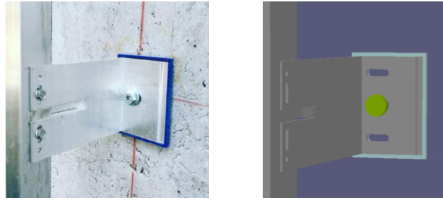
Figure 4 Detailed bracket in STL format
