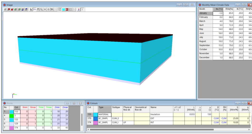
Figure 21. Material properties in TRISCO
