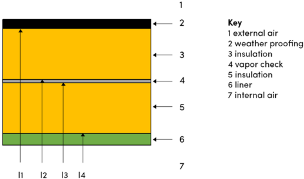
Figure 20. Layers and interfaces in roof
