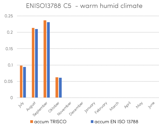
Figure 10. TRISCO results compared with the standard (condensation on interface 5)
