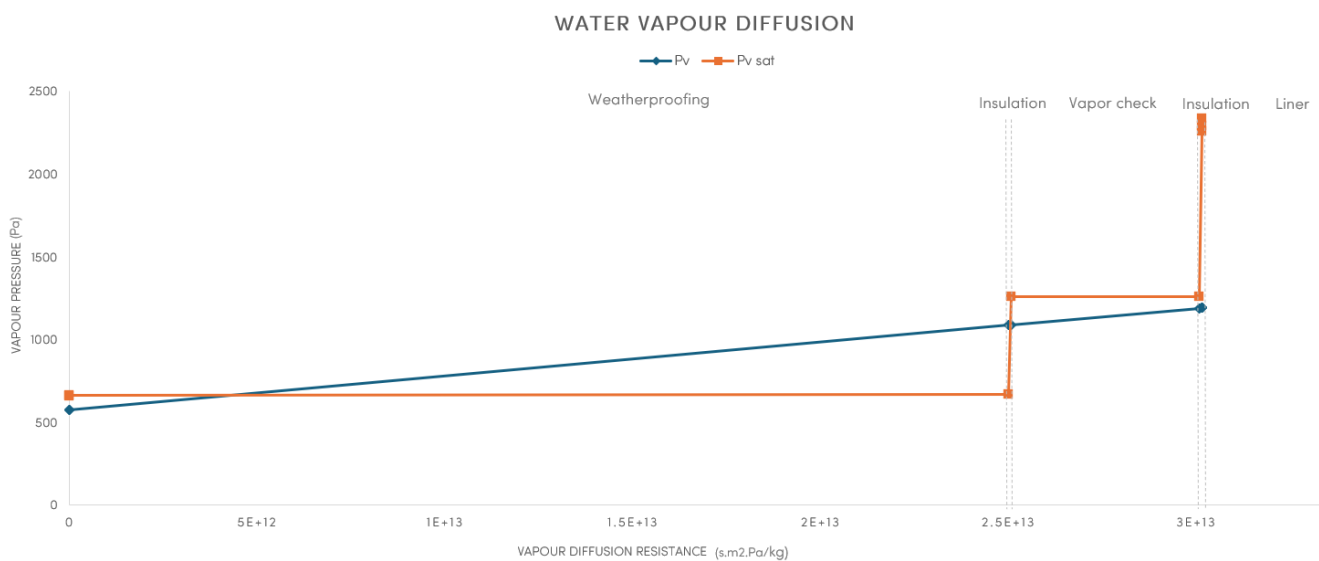
Figure 24. Result by Glaser method (December)
