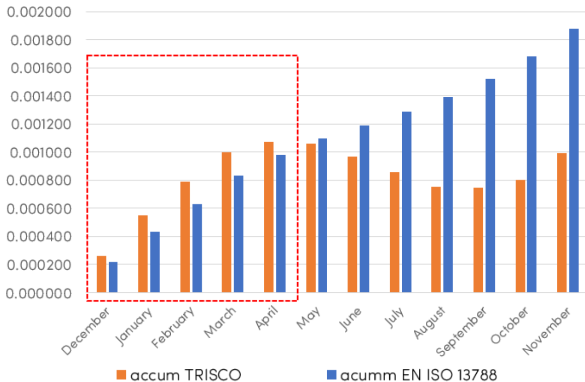
Figure 23. TRISCO and EN ISO 13788 accumulation rate
