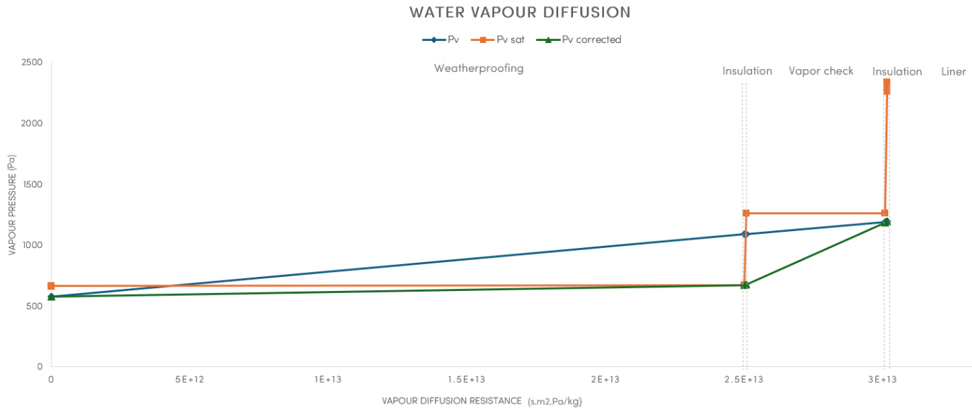
Figure 25. Corrected vapour pressure line
