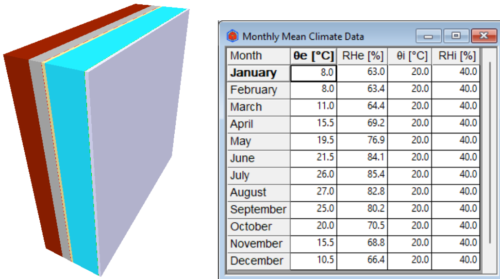
Figure 7. Geometry and climate in TRISCO
